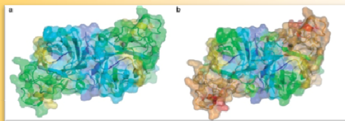
H/D-Ex of SOD1 WT
